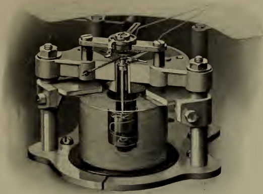
FIG. 25.—PHANTOM VIEW OF WESTON MODELS 151, 155, 156, 159, 160. Moving Parts of "Movable-Iron" Voltmeters.
